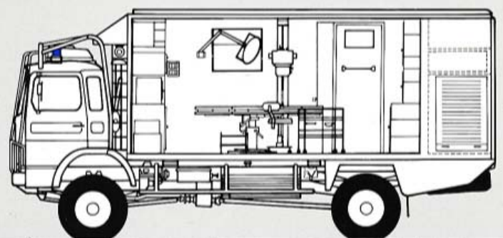
JE 13 - 4 x 4 Clinique mobile Mobile surgical unit
