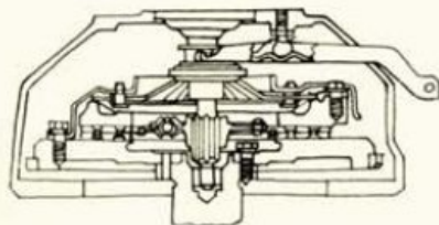
Clutch cutaway
