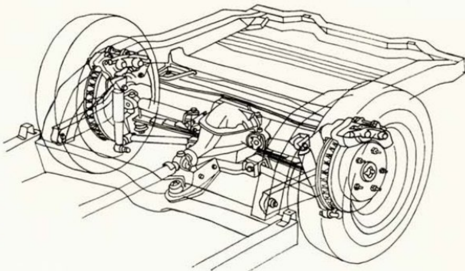
Rear suspension
