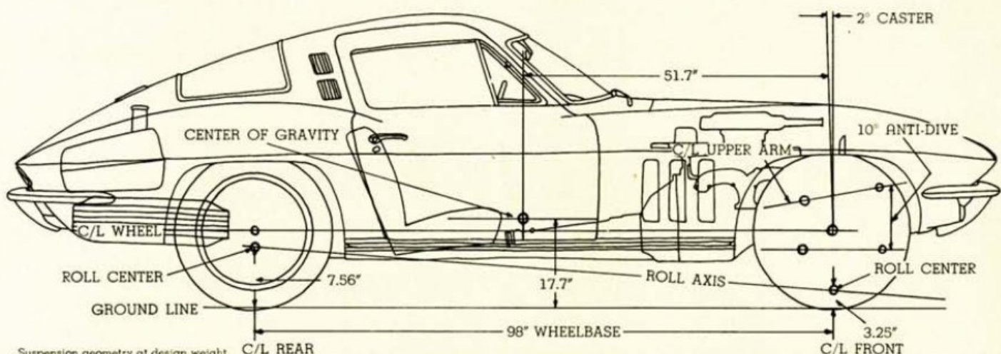
Suspension geometry at design weight
