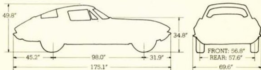
External dimensions, Sport Coupe
