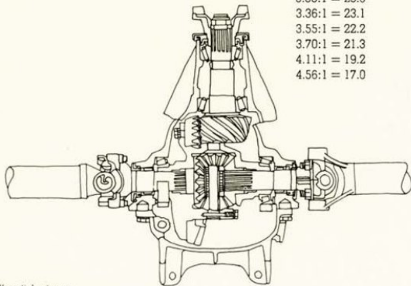
Differential cutaway
