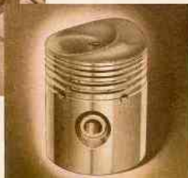
Here's the heart of Buick's Fireball principle. The special shape of this piston concentrates each fuel charge in ball-like shape before firing. Set off by the spark, this charge lets go with much smoother power than conventional design permits.
