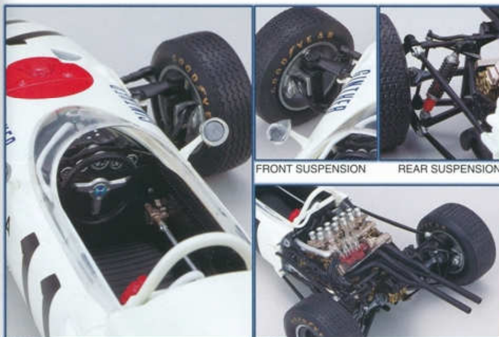
COCKPIT
